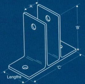
"H" BRACKET 2858
